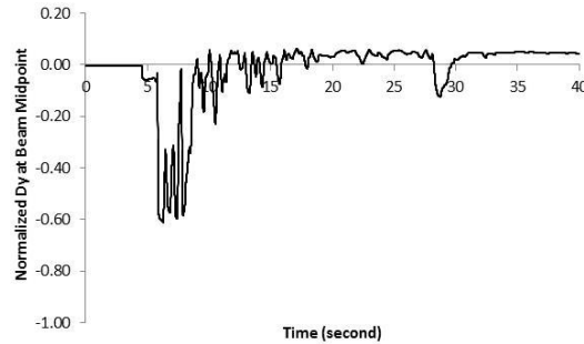
Figure 3.23. Beam ductility time history of the first story beam Combined strength ratio of each level columns time histories can be seen from Fig.3.24.
