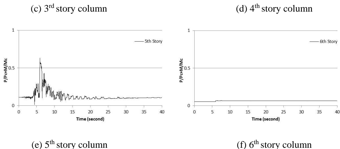
Figure 3.24. Combined strength ratio time history of columns of Frame F under GM13
