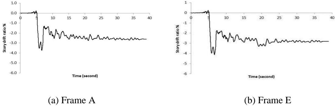
Figure 3.26. The first story drift ratio time histories of Frames A and E under GM11
