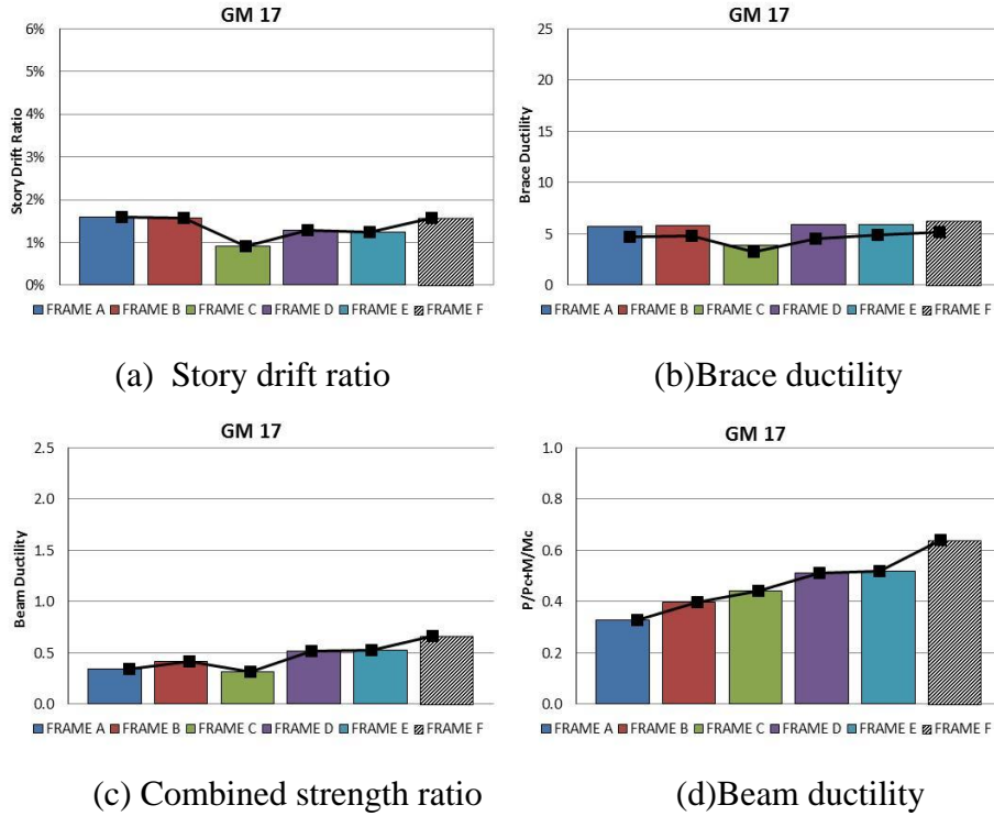
Fig. C17. Frame responses under GM17
