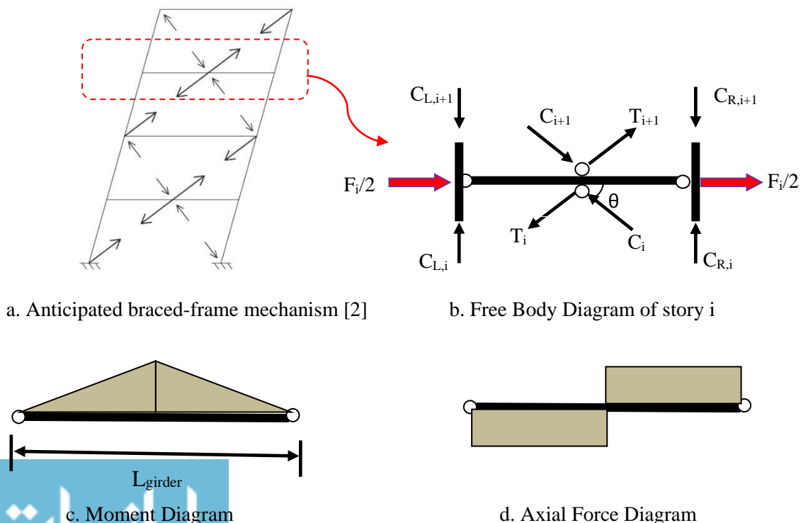
Fig. 2.2. Structural analysis of the brace-intersected girders in TSXBFs www.manaraa.com
