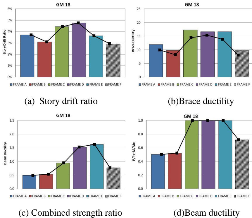
Fig. C18. Frame responses under GM18
