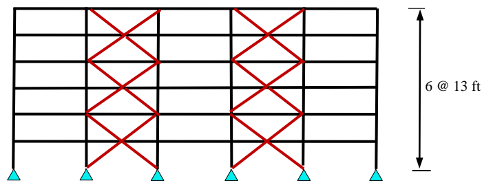
b. Elevation for frames having two-story X bracing configuration
