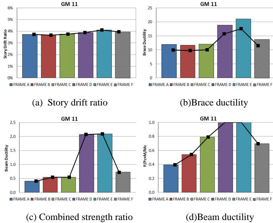
Fig. C11. Frame responses under GM11
