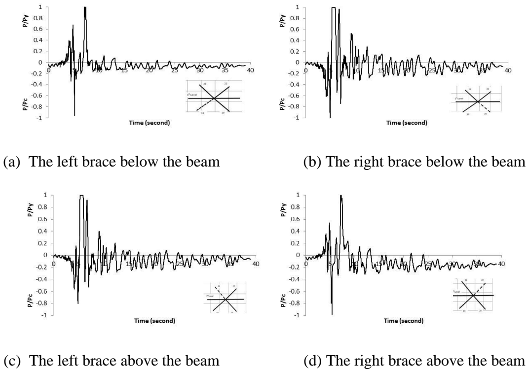
Figure 3.27. Normalized axial force time histories of the braces above and below the first story beam of Frame A
