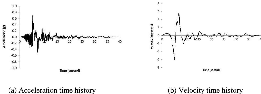
Figure 3.25 Acceleration and velocity time history of GM11
