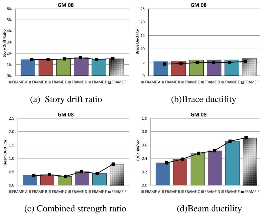
Fig. C8. Frame responses under GM08
