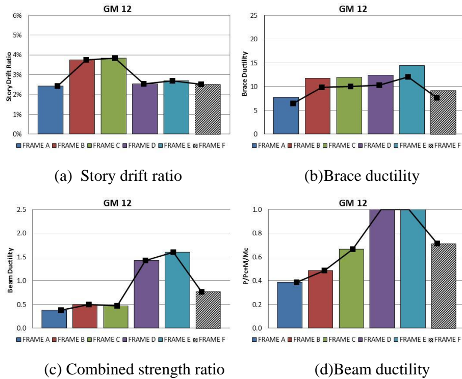
Fig. C12. Frame responses under GM12
