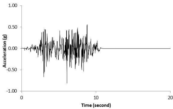
Fig. A9. Acceleration time history of GM9
